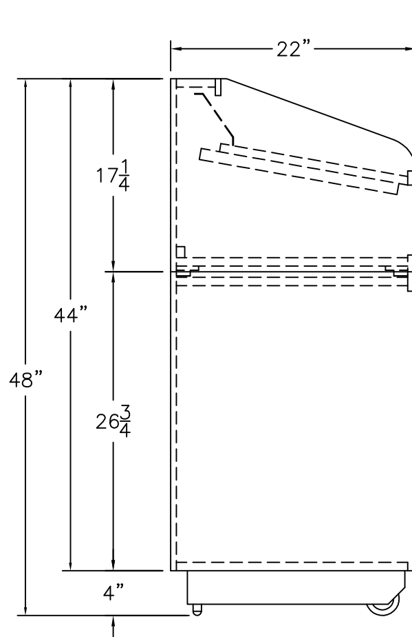
SIDE VIEW
