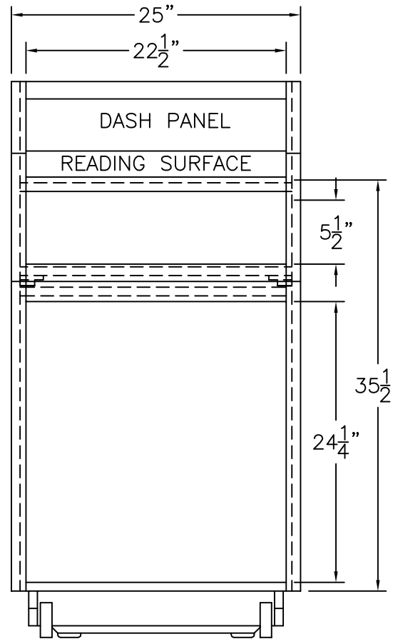
BACK VIEW
