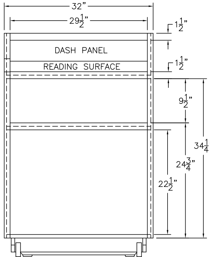
BACK VIEW
