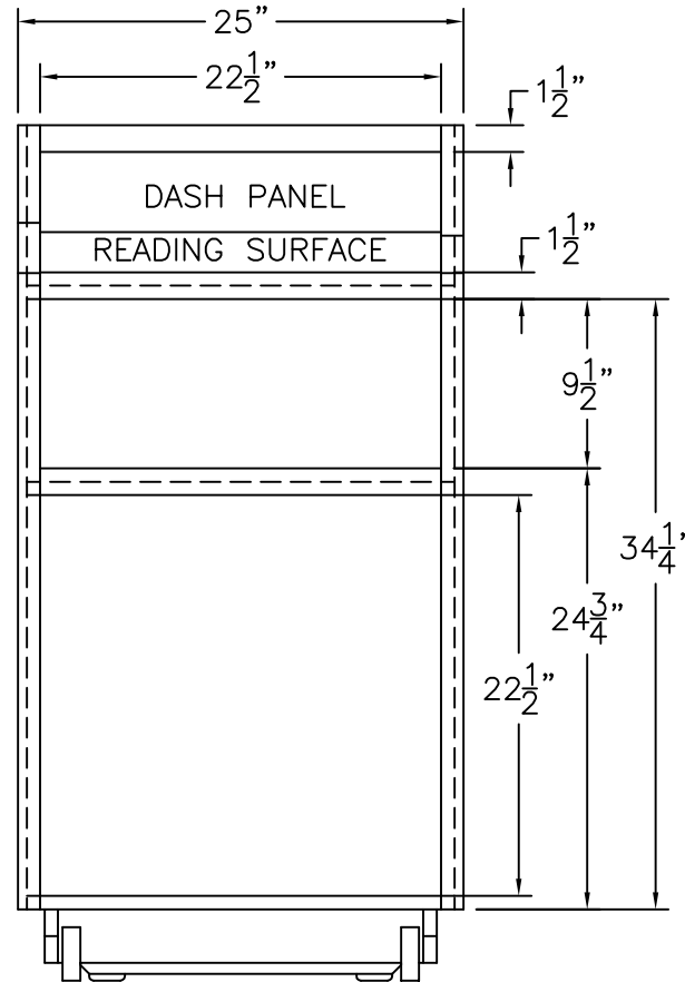
BACK VIEW
